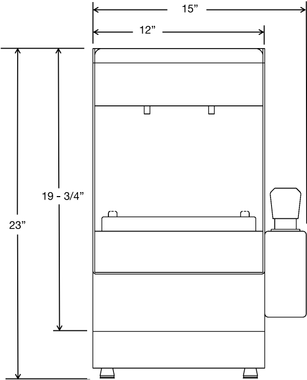
FRONT ELEVATION
